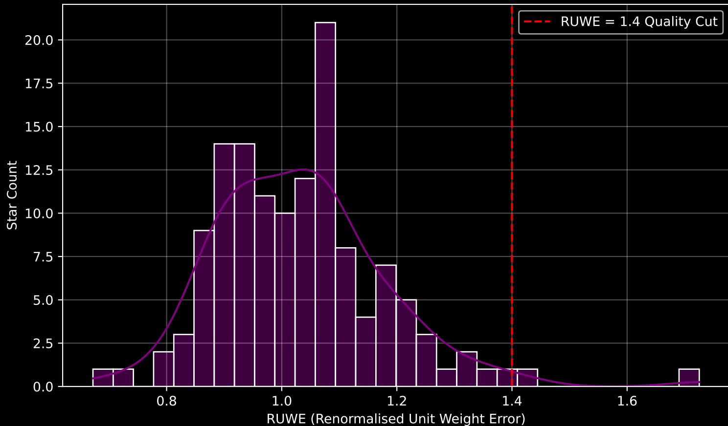
GAPOGEE DR17 Field [022+02] RUWE Distribution (n= 132)
