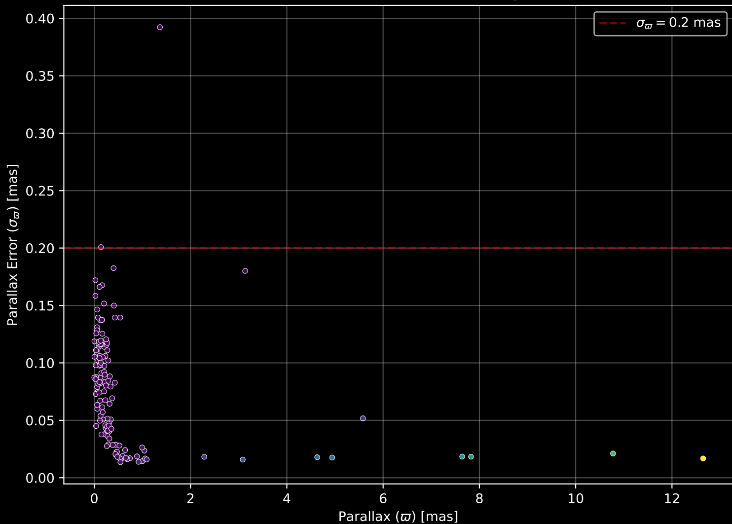
APOGEE DR17 Field: [022+02] Parallax Quality (n= 134)
