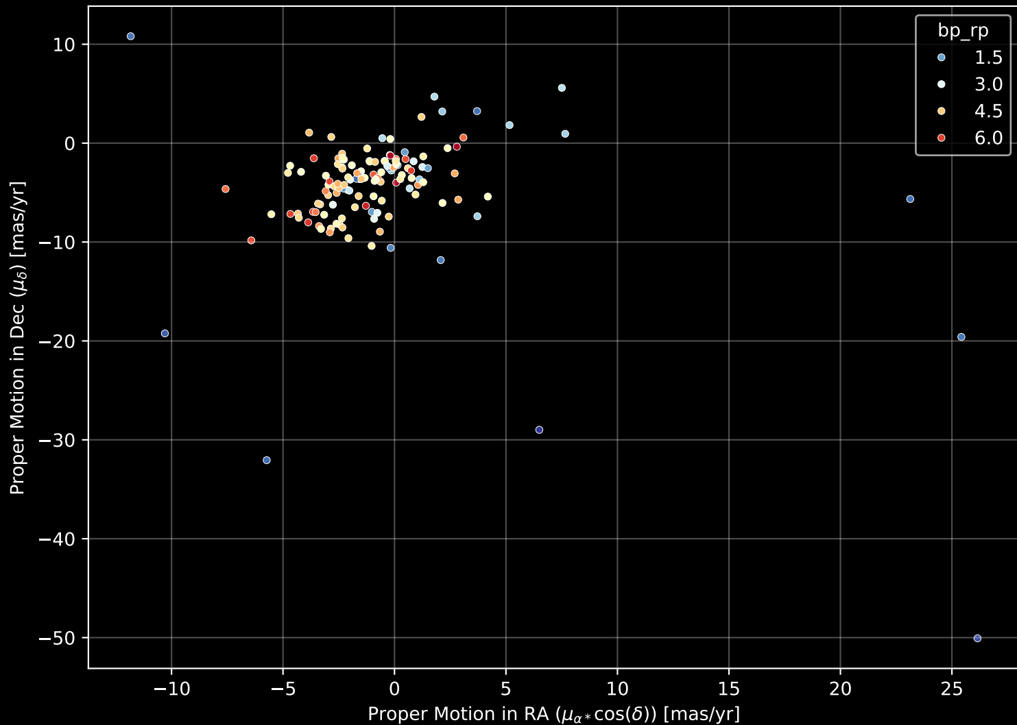
APOGEE DR17 Field: [022+02] Proper Motion Diagram (n= 134)
