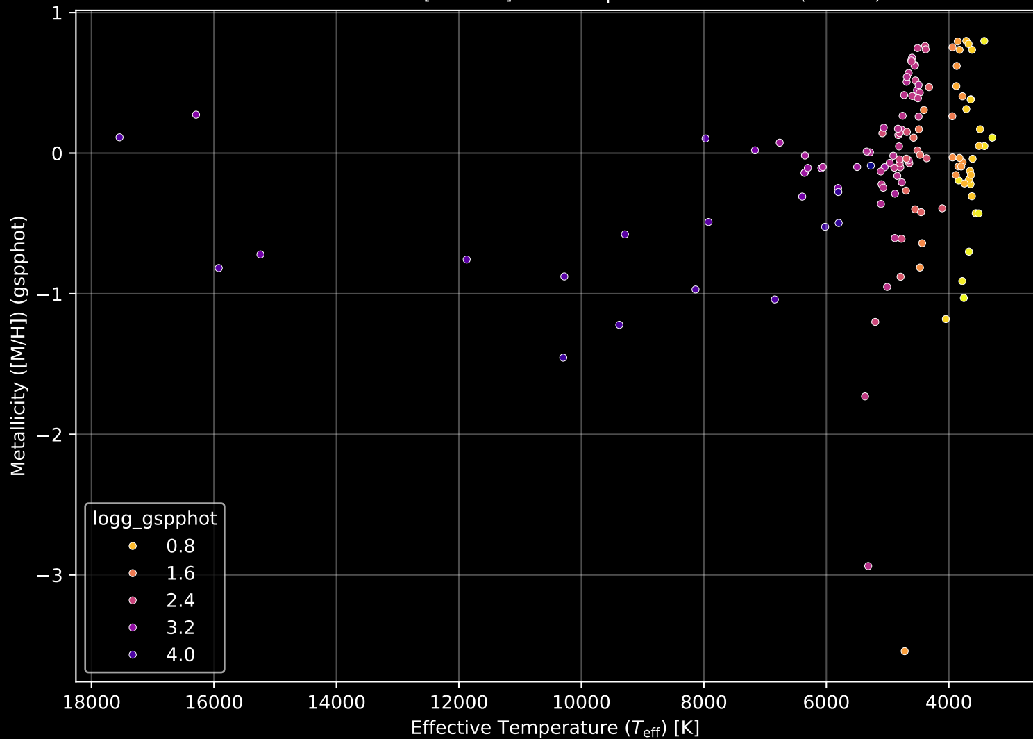
APOGEE DR17 Field: [022+02] Stellar Population Parameters (n= 134)
