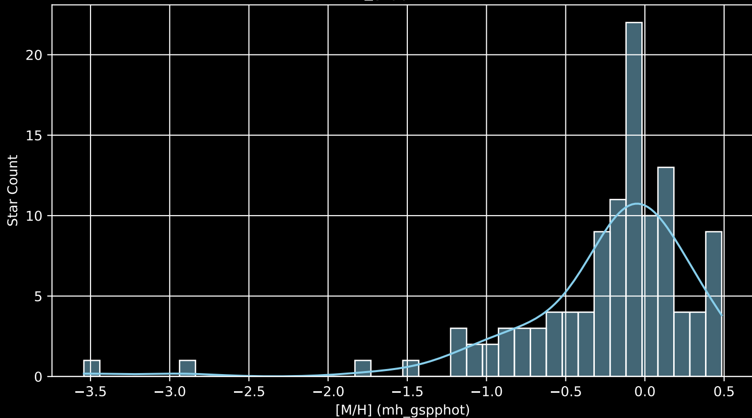
APOGEE DR17 Field: [022+02] [M/H] (mh_gspphot) (n= 114)
